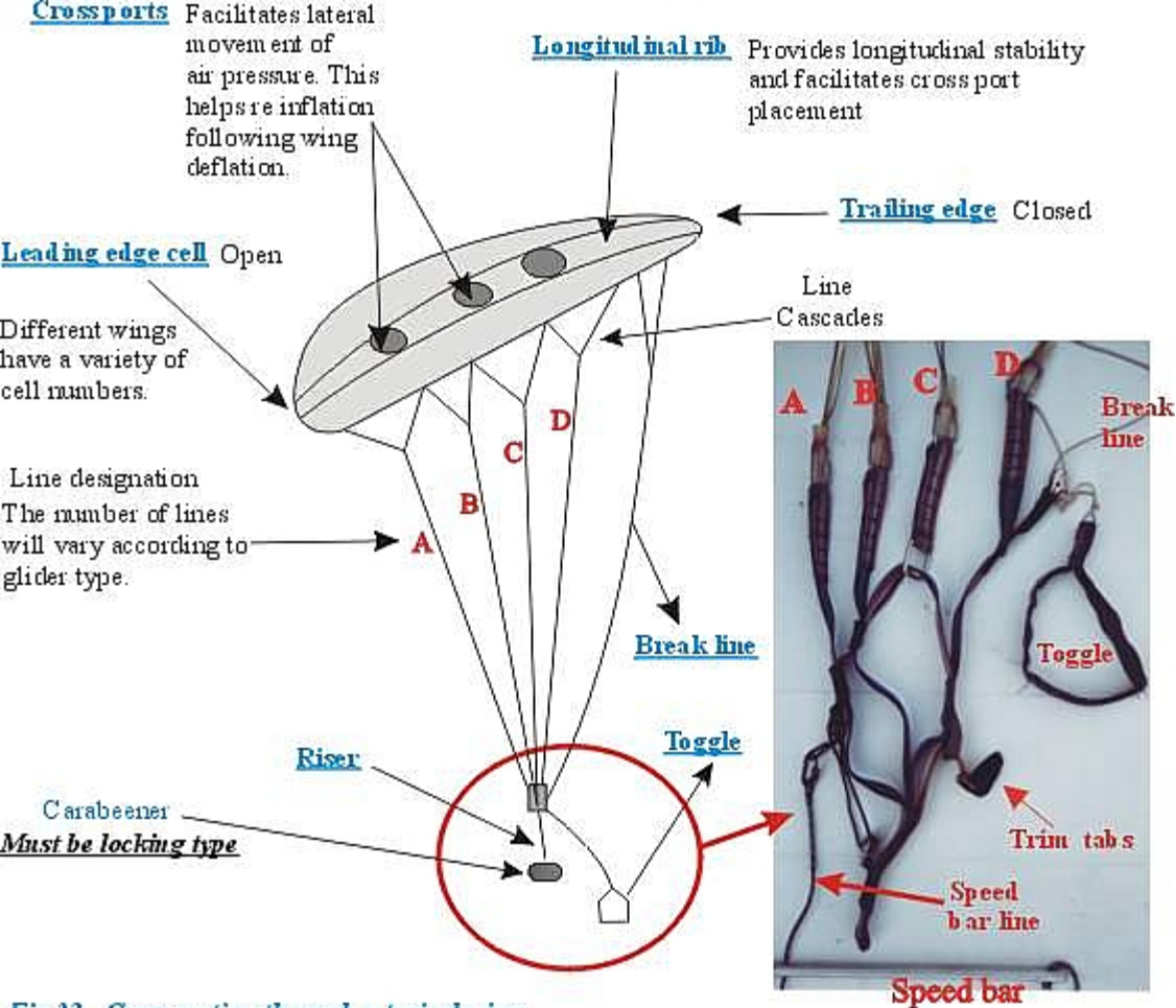
Fig 32 Cross section through a typical wing
